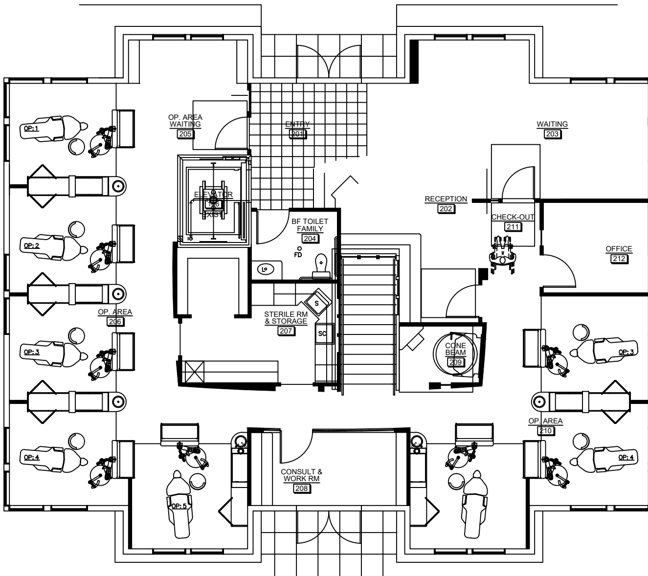
SECOND STORY FLOOR PLAN BUILDING #5
